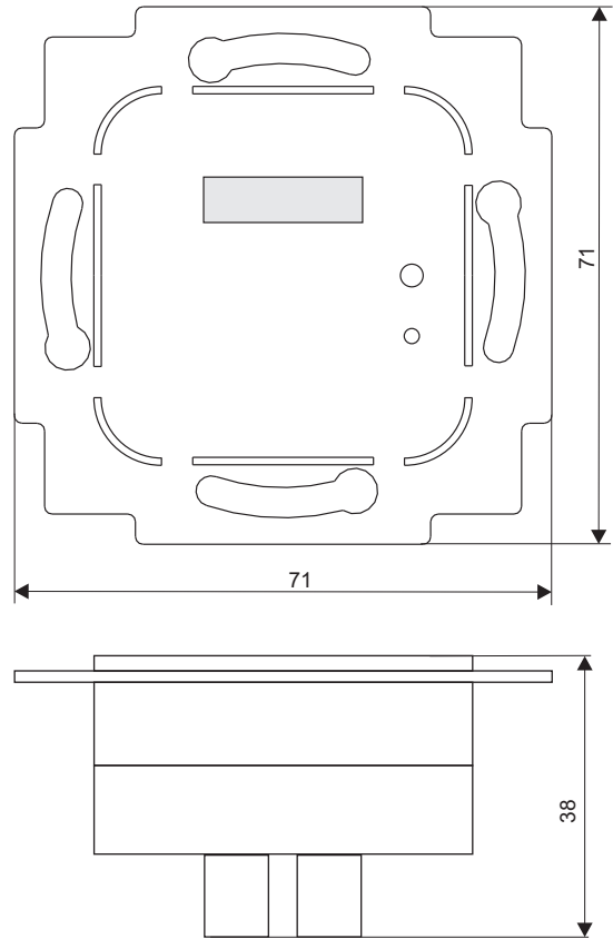
LON-Interface
